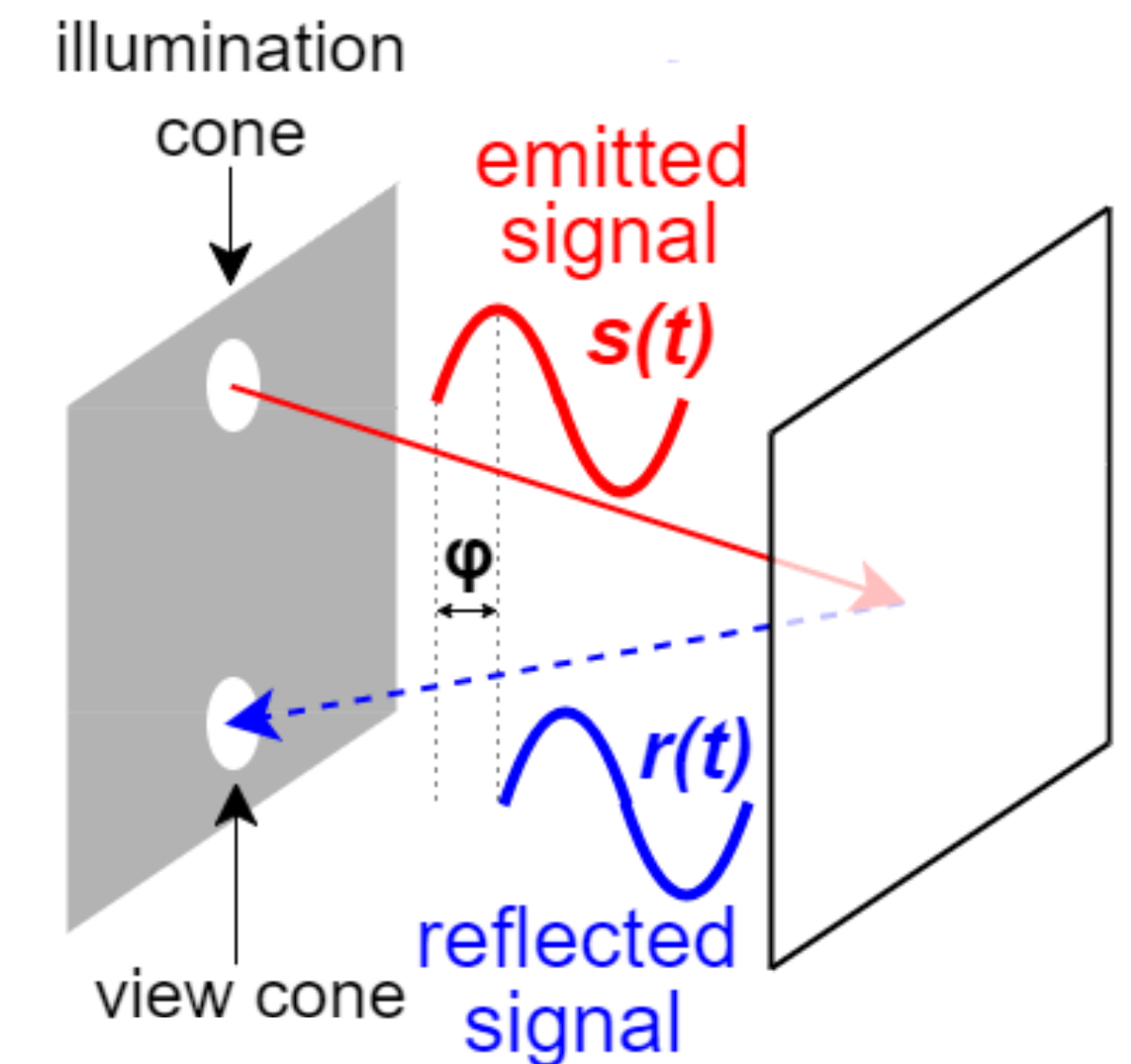
IR-ToF proximity sensor
